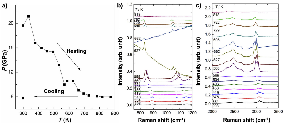
Fig. 7. (a) Temperature and pressure curve during the whole experiment of cyclohexane. (b, c) Selected Raman spectra of cyclohexane with increasing temperature at 19.7 GPa.
