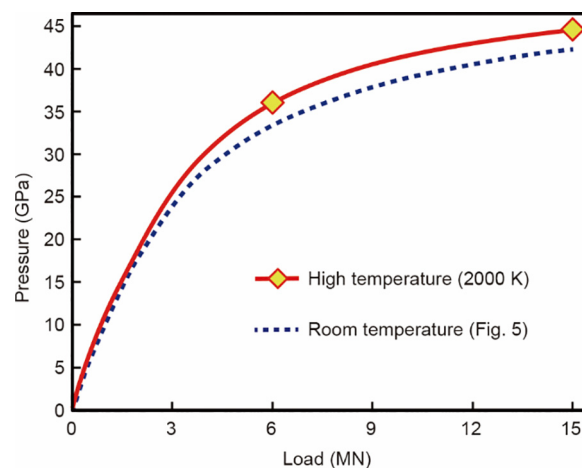
Fig. 6. Pressure generation using 1.5 mm TEL anvils with 1^\circ tapering (TF05 grade) at room temperature (dashed blue curve) and at a high temperature of 2000 K (solid red curve). The cell assembly shown in Fig. 4(b) was used for the high-temperature pressure generation test.
