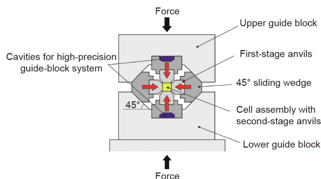
Fig. 1. Schematic drawings of the Osugi (DIA)-type compression system. A uniaxial press compresses guide blocks and finally creates a cubic compression space surrounded by six first-stage anvils, each of which compresses the cubic space in the [100] directions. Cavities are made in a KMAP with the high-precision guide-block system.
