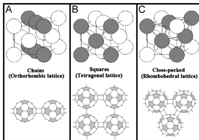
Fig. 3. Basic structures of the three low-dimensional phases of C_{60} . (Reprinted with permission from B. Sundqvist [20]).
