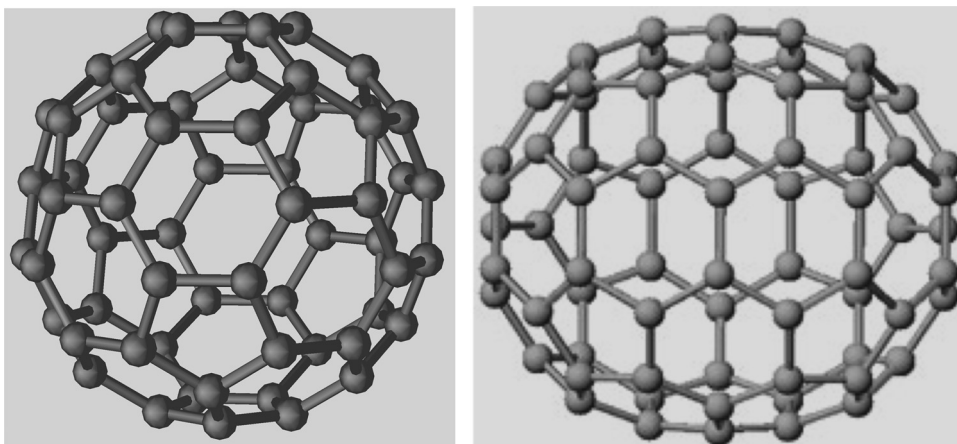
Fig. 1. The structures of C_{60} and C_{70} molecules.
