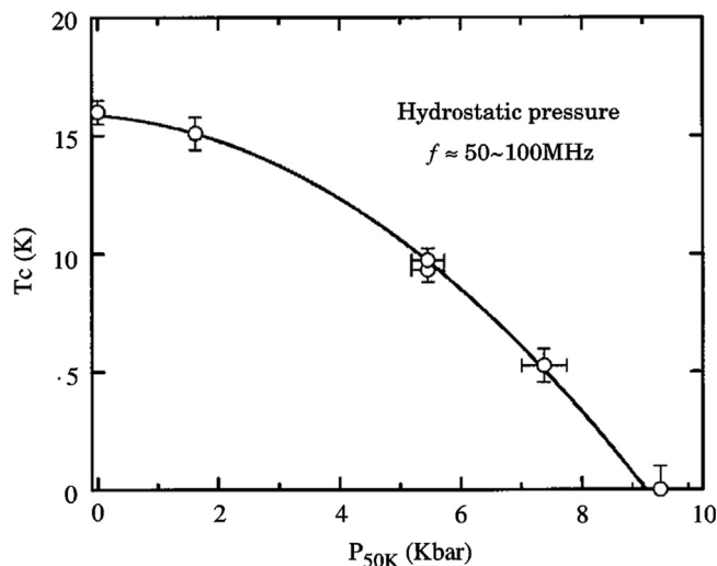
Fig. 7. T_c versus P_{50K} in C_{60} *TDAE. The solid curve indicates the theoretical prediction with the data up to 7.4 kbar. (Reprinted with permission from Mizoguchi et al. [56]).
