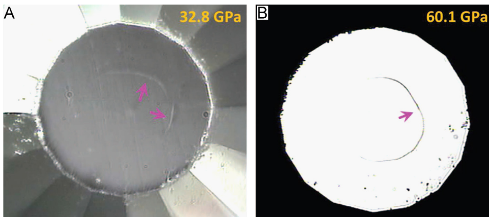
Fig. 11. Optical pictures of the ring cracks in the diamond anvils generated after formation of OACC and then release of the pressures from 32.8 GPa (A), and 60.1 GPa (B). (Reprinted with permission from Wang et al. [58]).
