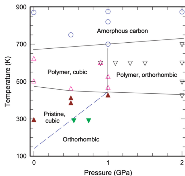
Fig. 9. Pressure–temperature phase diagram of C_{60}^*C_8H_8 . (Reprinted with permission from Iwasiewicz-Wabnig et al. [47]).
