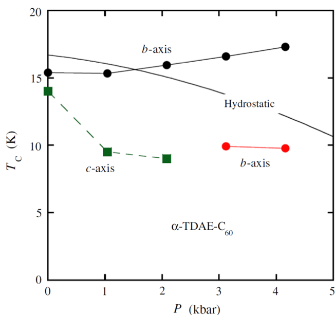
Fig. 8. T_c variations caused by uniaxial strain along b -axis [110] and c -axis, together with by hydrostatic pressure [111] (Reprinted with permission from Mizoguchi et al. [57]).
