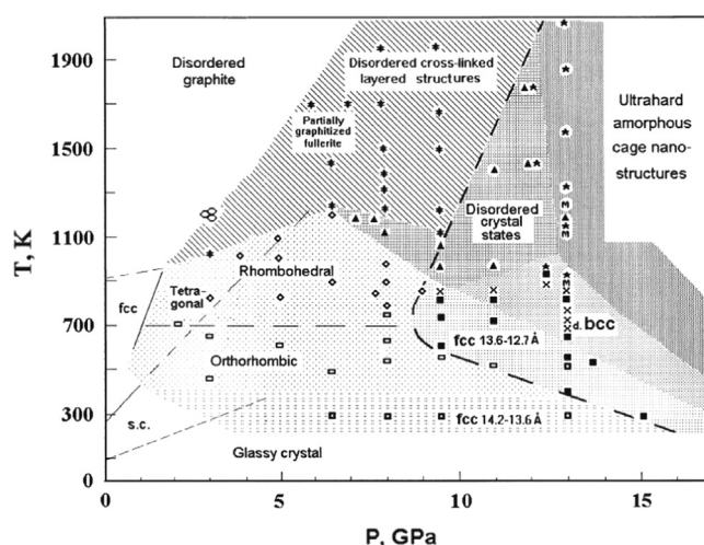
Fig. 2. Phase diagram of C_{60} showing the structural phases obtained under the pressure–temperature conditions shown. (Reprinted with permission from B. Sundqvist [20]).
