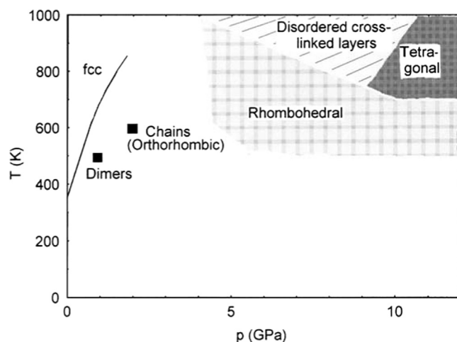
Fig. 4. Pressure–temperature phase diagram of C_{70} . (Reprinted with permission from B. Sundqvist [20]).
