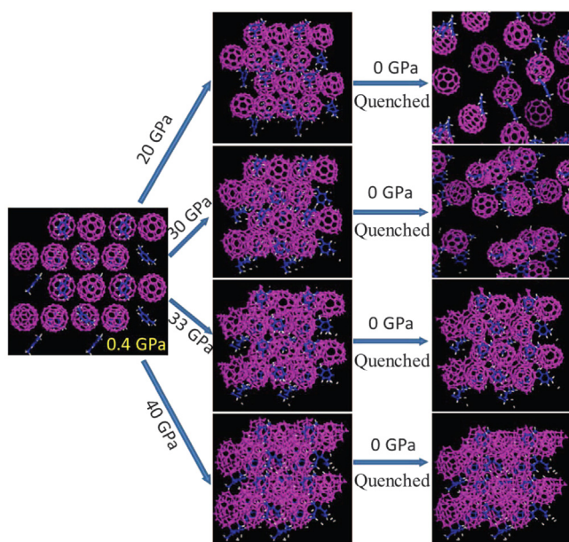
Fig. 10. Simulated structures of the material under different compression and decompression conditions. (Reprinted with permission from Wang et al. [58]).
