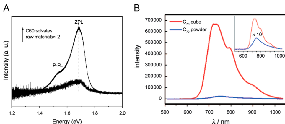
Fig. 6. PL spectra of C_{60} *m-xylene solvate and pristine C_{60} (A), and C_{70} *2mesitylene solvate and pristine C_{70} powder (B). (Adapted from [28] and [102]).
