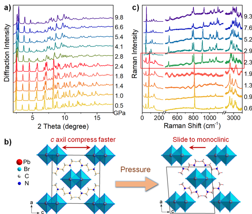
Figure 2. Structural transformation of C_4N_2H_{14}PbBr_4 under pressure. (a) In situ XRD patterns. (b) Crystal structure viewing along the 1D chain direction ( b axis), which illustrates the orthorhombic to monoclinic phase transition at 2.8 GPa. (c) Raman spectra.
