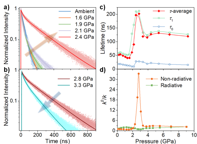
Figure 3. Time-resolved PL of C_4N_2H_{14}PbBr_4 under pressure: (a) 0–2.4 GPa; (b) 2.8 and 3.3 GPa. (c) The PL lifetime as a function of pressure. (d) Suppression of radiative and nonradiative recombination rates ( k_r^0/k_r and k_{nr}^0/k_{nr} ) under high pressure.
