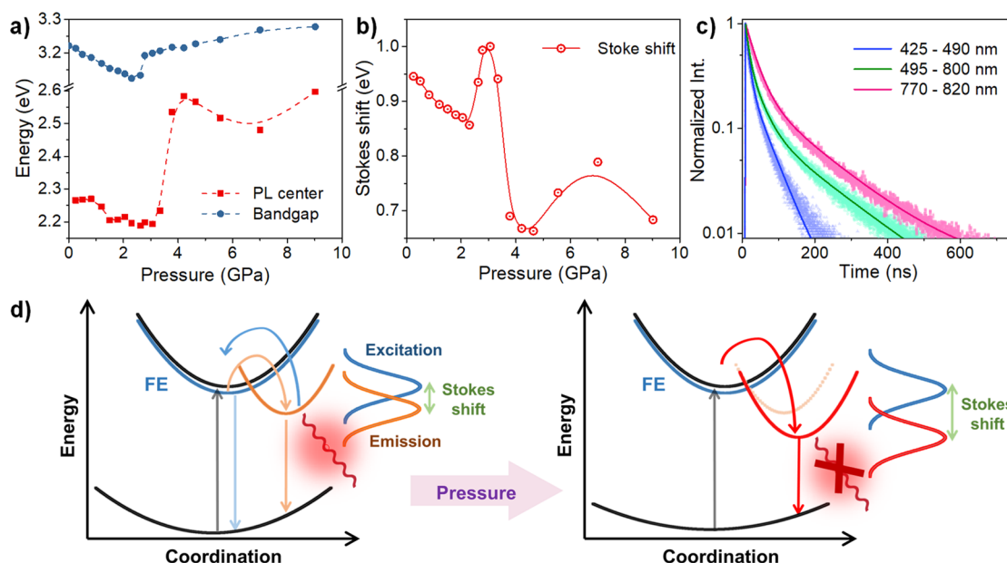
Figure 4. (a) Pressure-induced evolution of bandgap and PL emission energy. (b) Stokes shift of C_4N_2H_{14}PbBr_4 under high pressure. (c) Comparison of the PL decay at different wavelength ranges using an optical filter at 2.1 GPa, which implies that the excitons possessing a higher binding energy exhibit a longer lifetime and possibly smaller k_{nr} . (d) Schematic illustration of the pressure-induced changes in the STE and Stokes shift. STEs would be more stable under a suitable pressure, to result in a larger Stokes shift and more localized excitons that have less chance to encounter defects. In addition, with increasing STE binding energy, the population of STEs increased while the free exciton (FE) states reduced, as evidenced by the disappearance of the FE emission beyond 2.3 GPa (Figure S2).
