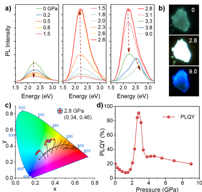
Figure 1. Pressure-dependent PL of C_4N_2H_{14}PbBr_4 under 360 nm excitation. (a) In situ PL spectra at different pressures. (b) PL photographs at selected pressures: ambient (top), 2.8 GPa (middle), and 9.0 GPa (bottom). (c) Chromaticity coordinates of the emissions under different pressures, which show a wide range of color tunability. (d) Evolution of PLQY during compression.
