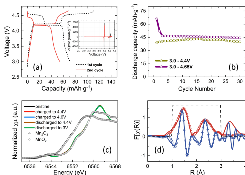
Figure 2. (a) Charge/discharge curves of the initial two cycles of Na 2 Mn 3 O 7 at a cycling rate of C/20 with the corresponding dQ/dV plots shown as an inset. (b) Cycling performance under a rate of C/10 within two different voltage windows. (c) XANES part of Mn K-edge XAS spectra for the pristine and charged samples (charged to 4.4 and 4.6 V, discharged to 4.4 and 3.0 V). Reference spectra of Mn 2 O 3 and MnO 2 are also shown to indicate the valence state of the samples, all of which are tetravalent (have similar character to MnO 2 ). (d) Fitting to both the magnitude and the real part of Fourier-transformed EXAFS spectrum of the pristine sample.
