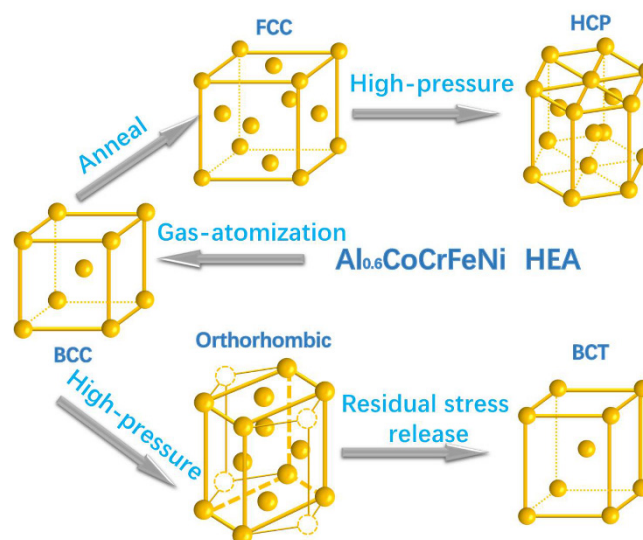
Figure 7. A schematic illustration of the atomic structure for five polymorphs observed in the \text{Al}_{0.6}\text{CoCrFeNi} HEA and the transition paths between them [62].
