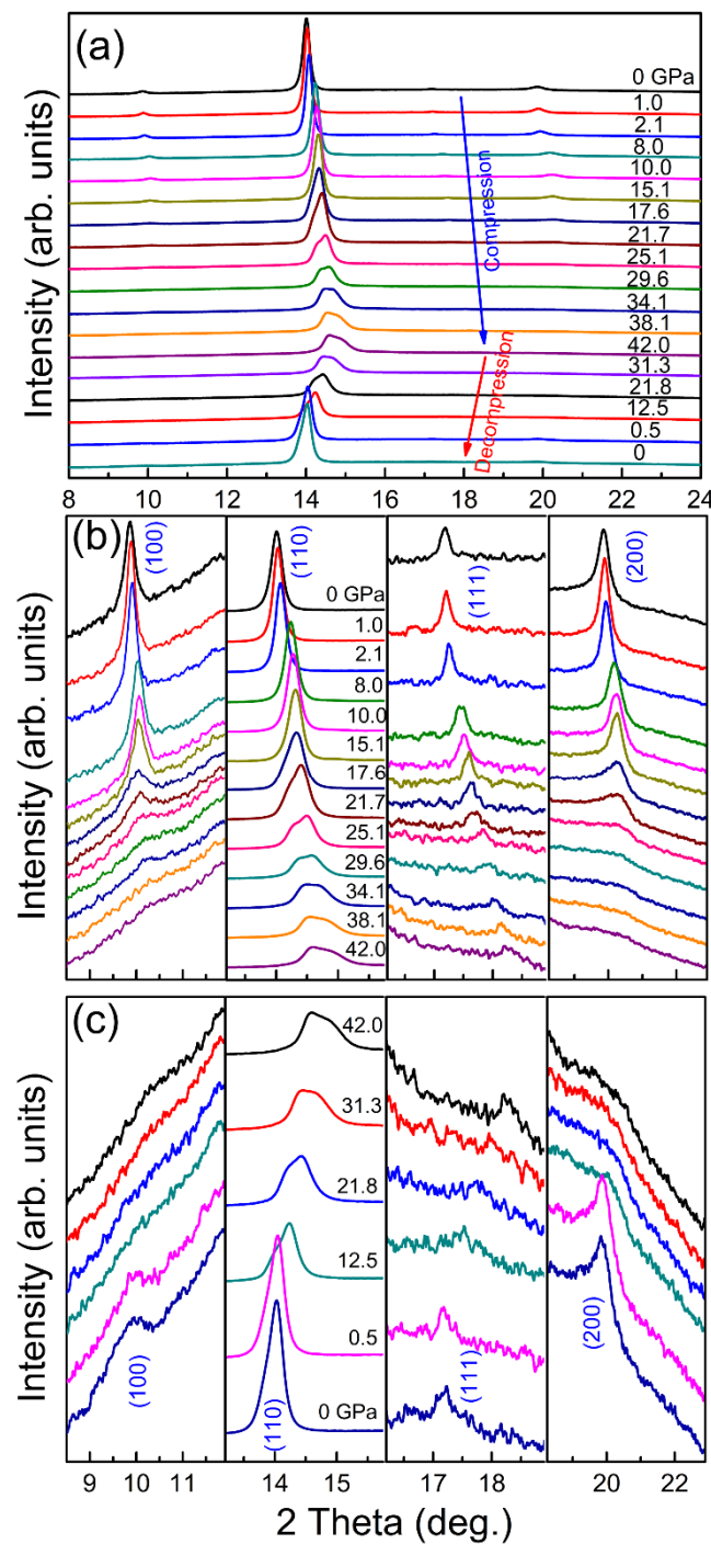
Figure 6. The structural evolution of the AlCoCrFeNi HEA as a function of pressure monitored by in situ high-pressure XRD patterns at room temperature (a) and the locally enlarged plot of the XRD patterns for each peak upon compression (b) and decompression (c) to show more details of the peak shape and width: The x-ray wavelength is 0.4959 Å [61].
