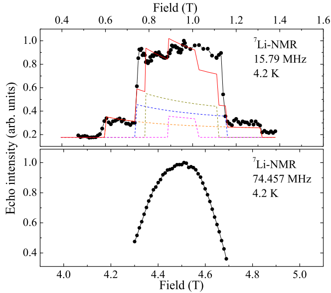
FIG. 9. (Color online) The ^7\text{Li} spectrum for \text{Li}_3\text{Ni}_2\text{SbO}_6 at 4.2 K in antiferromagnetic phase at different magnetic fields: 0.95 T for upper panel and 4.5 T for lower panel. Red line is the result of dipole-dipole calculations; dashed lines are the calculated contributions of different magnetically nonequivalent Li positions in the frame of the powder averaging of the zigzag model.
