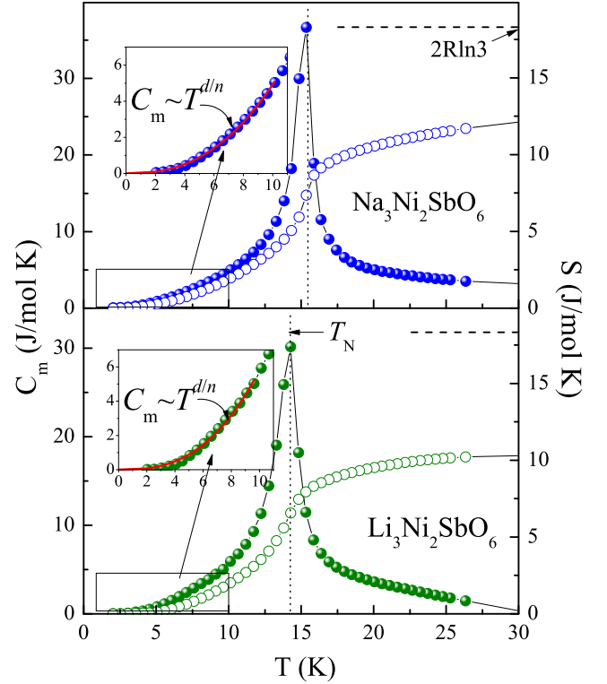
FIG. 6. (Color online) Magnetic specific heat (filled circles) and magnetic entropy (open circles) for \text{A}_3\text{Ni}_2\text{SbO}_6 at B = 0 T. Insets: Enlarged low-temperature parts with solid curve indicating the spin-wave contribution estimated in accordance with a C_m \propto T^{d/n} power law for magnons.
