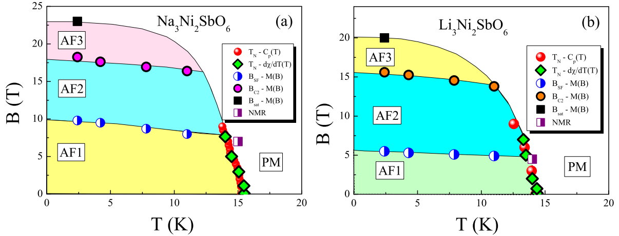
FIG. 12. (Color online) Magnetic phase diagrams for antimonates A_3\text{Ni}_2\text{SbO}_6 : (a) A = \text{Na} ; (b) A = \text{Li} .
