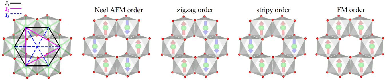
FIG. 1. (Color online) 2D honeycomb lattice Heisenberg model with up to third neighbor exchanges, J_{1,2,3} , and spin-configuration diagrams for Néel, zigzag, stripy, and ferromagnetic (FM) order.
