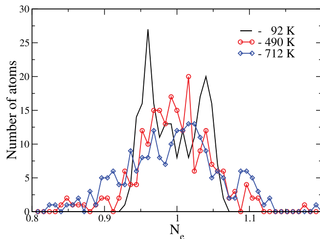
Figure 6 | Density of states for the charge distribution according to Bader procedure for Cmca-12 at 260 GPa. The DOS at 92 \text{ K} in non-diffusive state is narrow and asymmetric. The DOS in diffusive and liquid states are wide and similar implying similar electronic structure.
